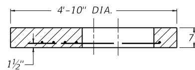
SECTION A-A FLAT SLAB TOP DETAIL
