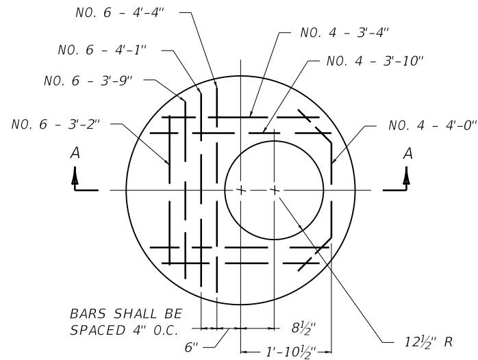
PLAN VIEW FLAT SLAB TOP DETAIL
