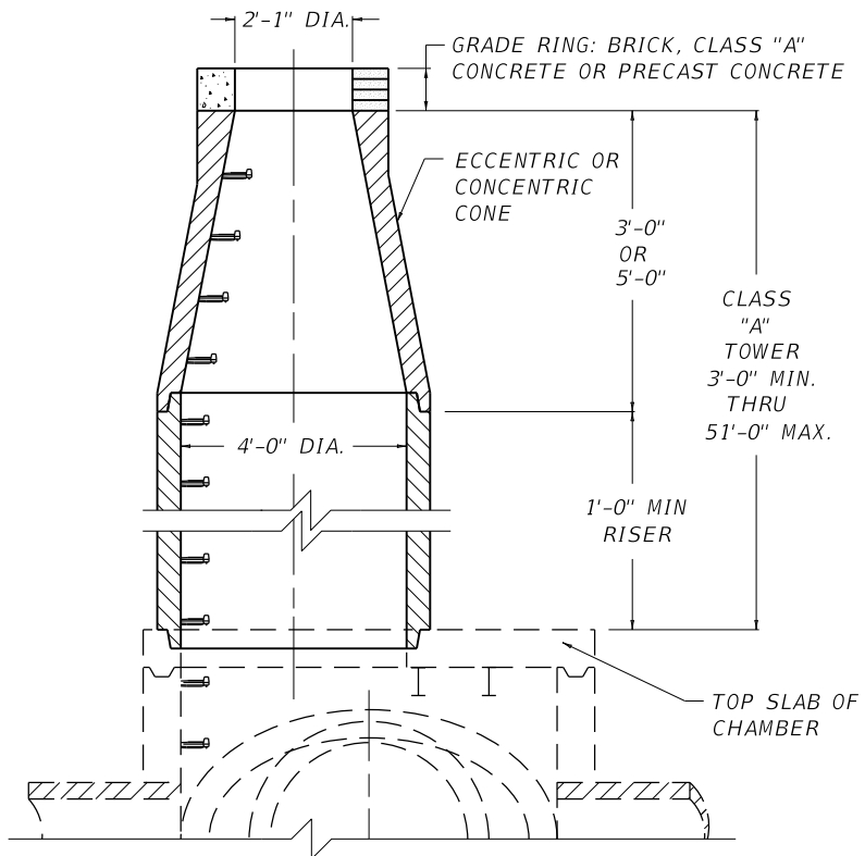
CLASS "A" TOWER DETAIL
